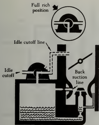
FIGURE 3-12. Back-suction type mixture control system.
